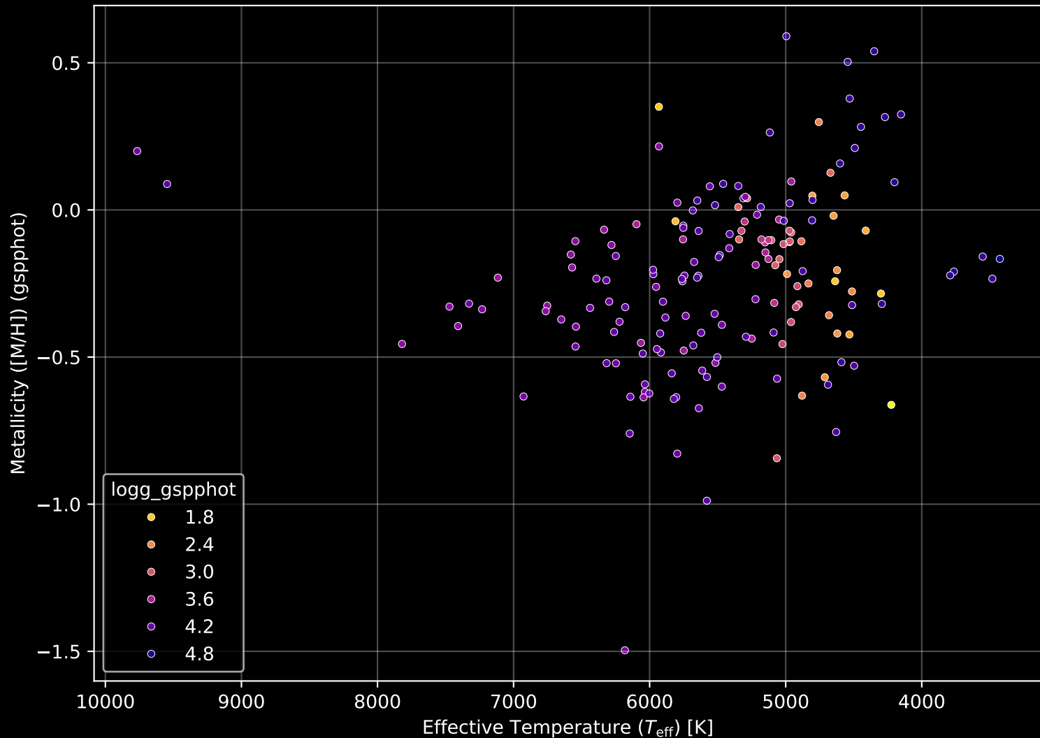
APOGEE DR17 Field: [056-37_MGA] Stellar Population Parameters (n= 171)
