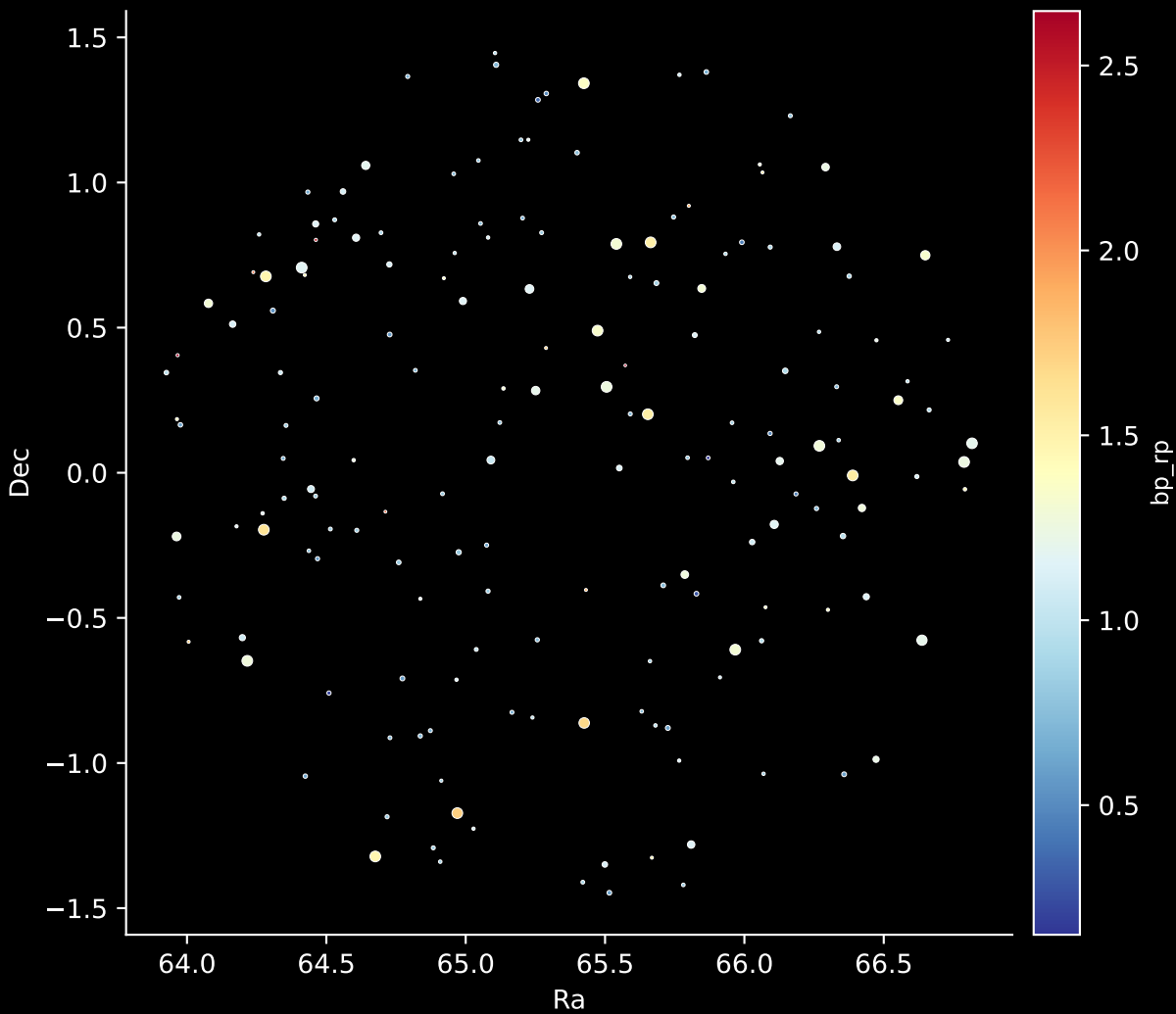
APOGEE DR17 Field: [056-37_MGA] Stars: 171
