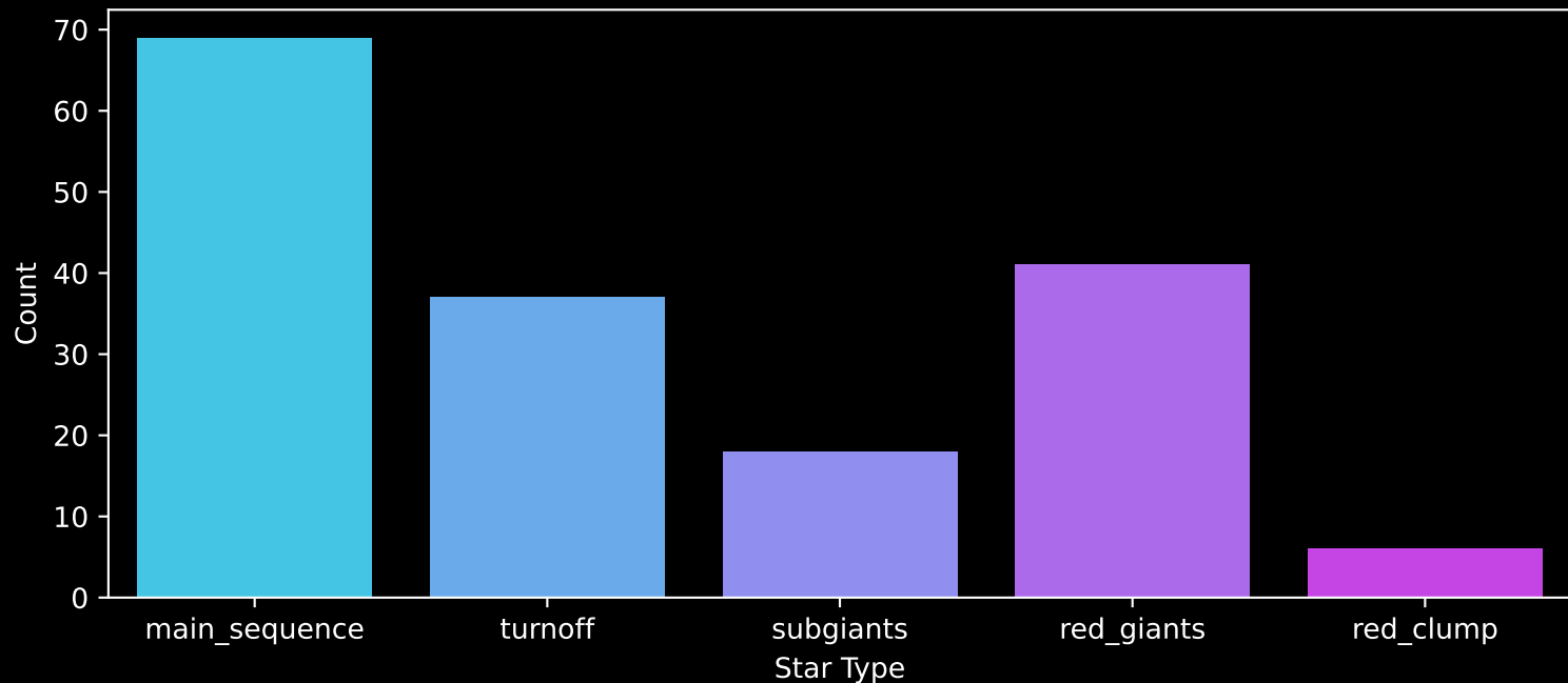
APOGEE DR17 Field: [056-37_MGA] Count plot of Star Type
