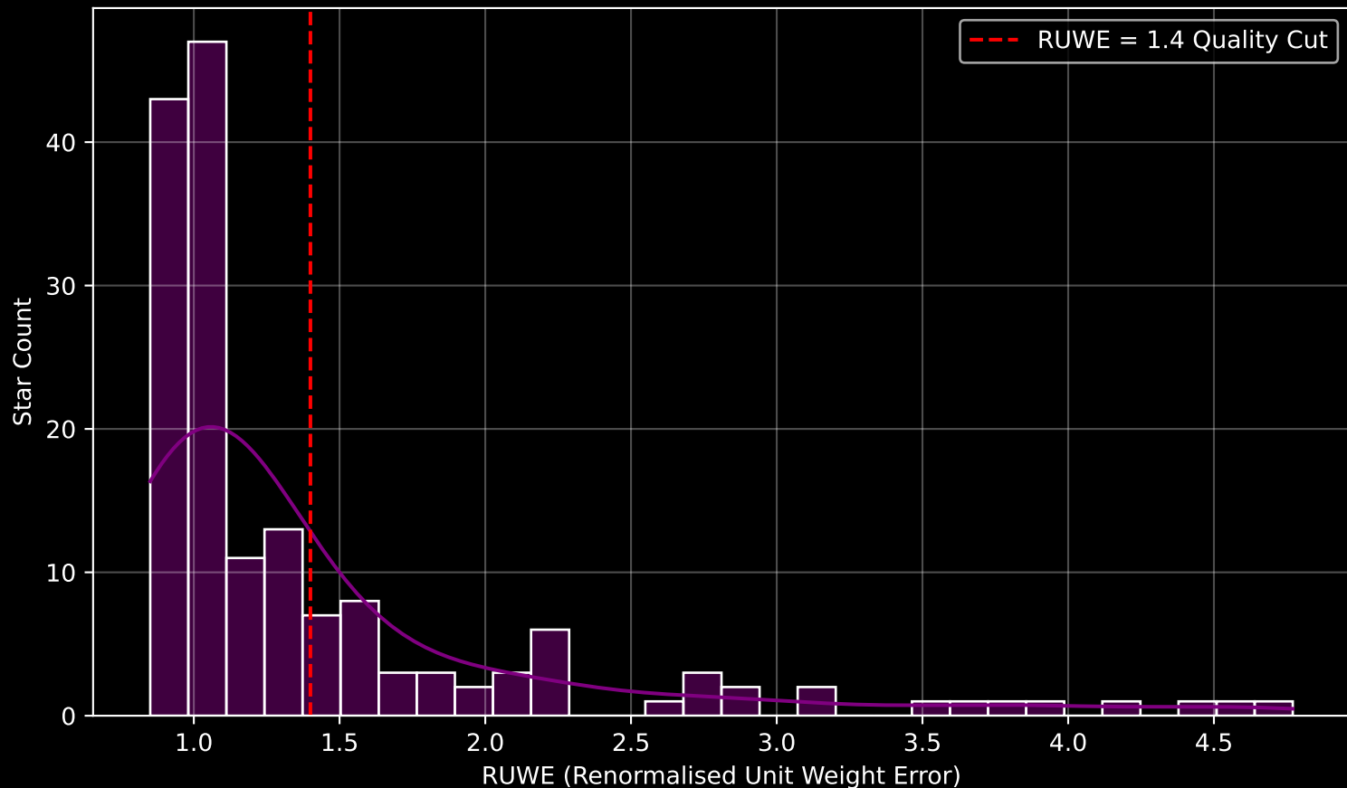
GAPOGEE DR17 Field [056-37_MGA] RUWE Distribution (n= 162)
