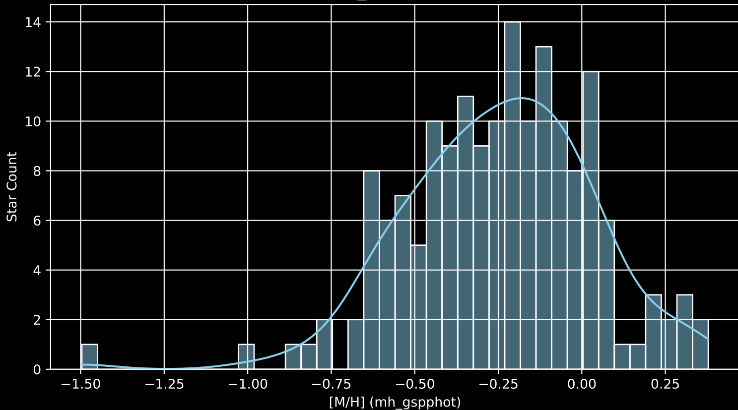
APOGEE DR17 Field: [056-37_MGA [M/H] (mh_gspphot) (n= 168)
