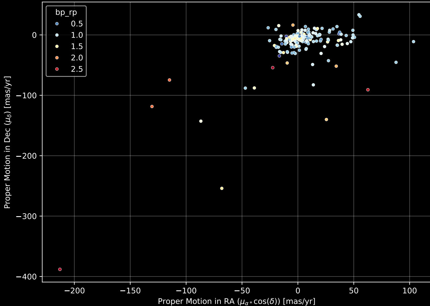
APOGEE DR17 Field: [056-37_MGA] Proper Motion Diagram (n= 171)
