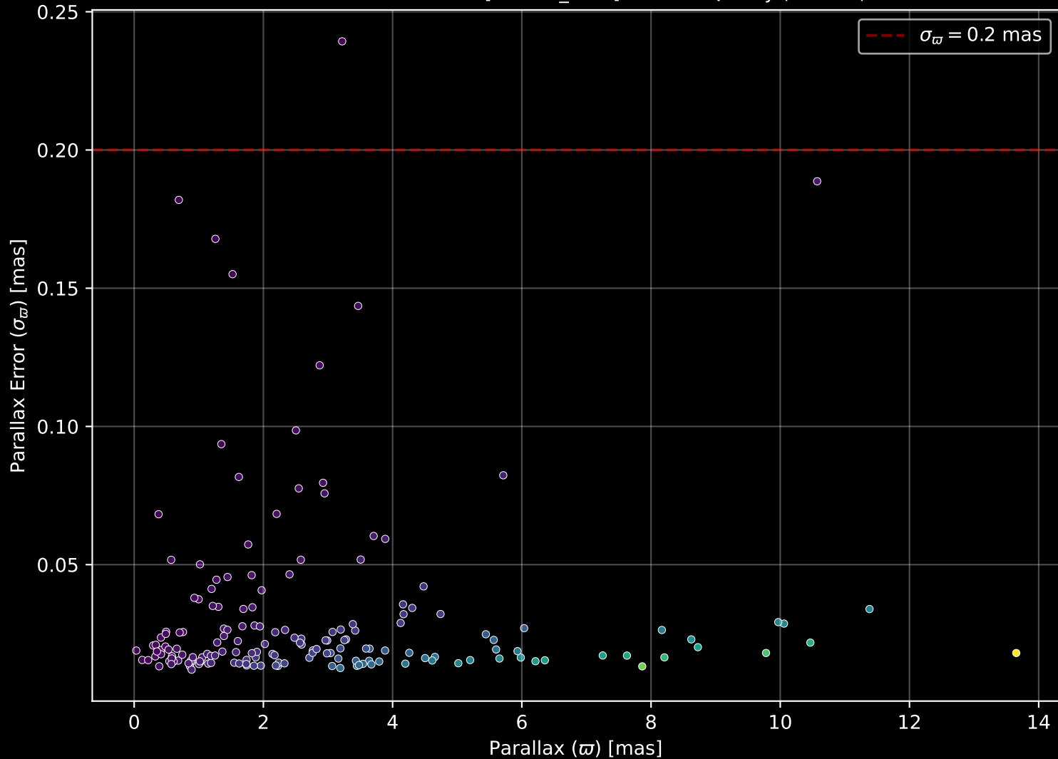
APOGEE DR17 Field: [056-37_MGA] Parallax Quality (n= 171)
